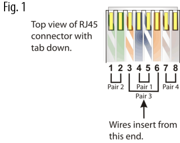
Fig. 1: EIA 568A and 568B wiring scheme for CAT5 Cable
